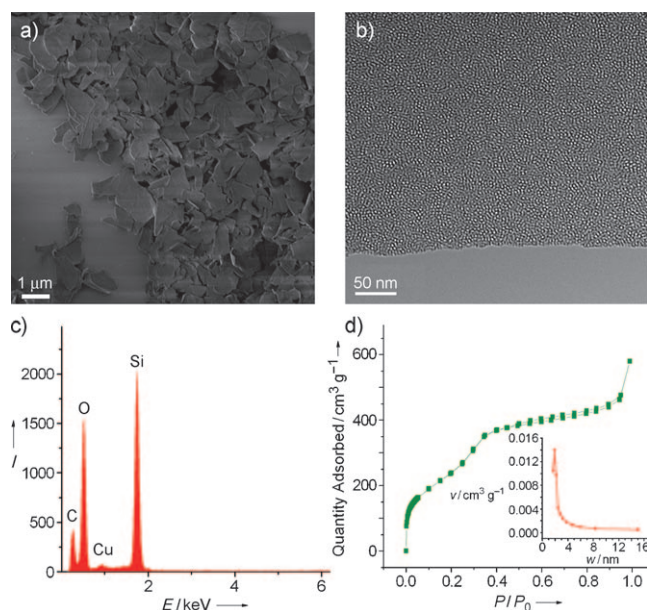
Figure 3. Graphene-based mesoporous silica (GM-silica) sheets after pyrolysis at 800°C. a) FE-SEM and b) TEM images reveal the stable morphology and mesoporous structure of GM-silica sheets after pyrolysis at high temperature. c) EDX spectrum, suggesting that graphene remains in GM-silica sheets. d) Nitrogen adsorption/desorption isotherm of graphene-mesoporous silica sheets (inset: pore size distribution), further demonstrating the mesoporous structure, with the pore size of 2 nm and BET surface area of 980 m 2 g -1 .
